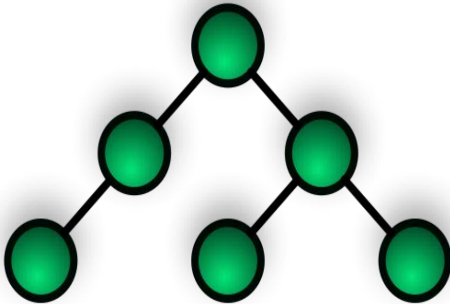
Tree Network
